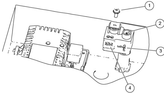
Tamper Arrangement
