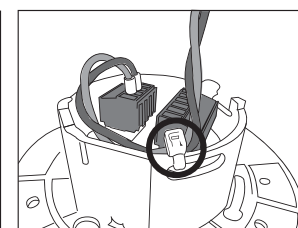
strain-relief
